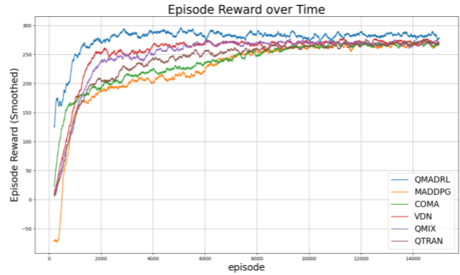
Figure 6. Reward variation of QMARL and multiple baseline algorithms.
