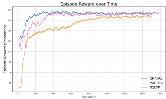
Figure 7. Reward variation before and after the introduction of the quantum experience replay module.
